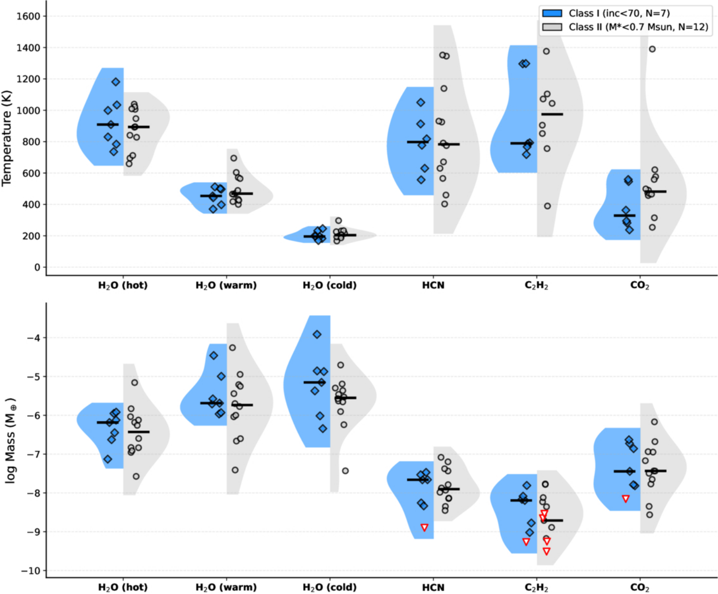
Figure 7. from Ke Zhang et al 2026 Astron. J. 172 doi:10.3847/1538-3881/ae90a1 https://dx.doi.org/10.3847/1538-3881/ae90a1 © 2026. The Author(s). Published by the American Astronomical Society.
