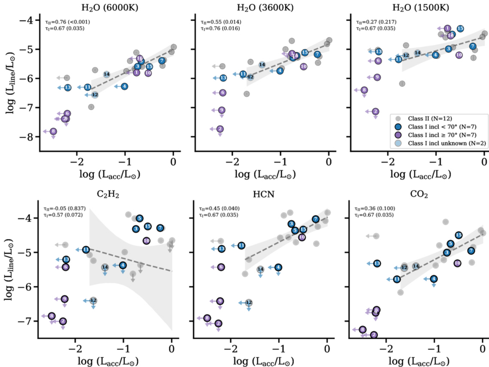
Figure 4. from Ke Zhang et al 2026 Astron. J. 172 doi:10.3847/1538-3881/ae90a1 https://dx.doi.org/10.3847/1538-3881/ae90a1 © 2026. The Author(s). Published by the American Astronomical Society.
