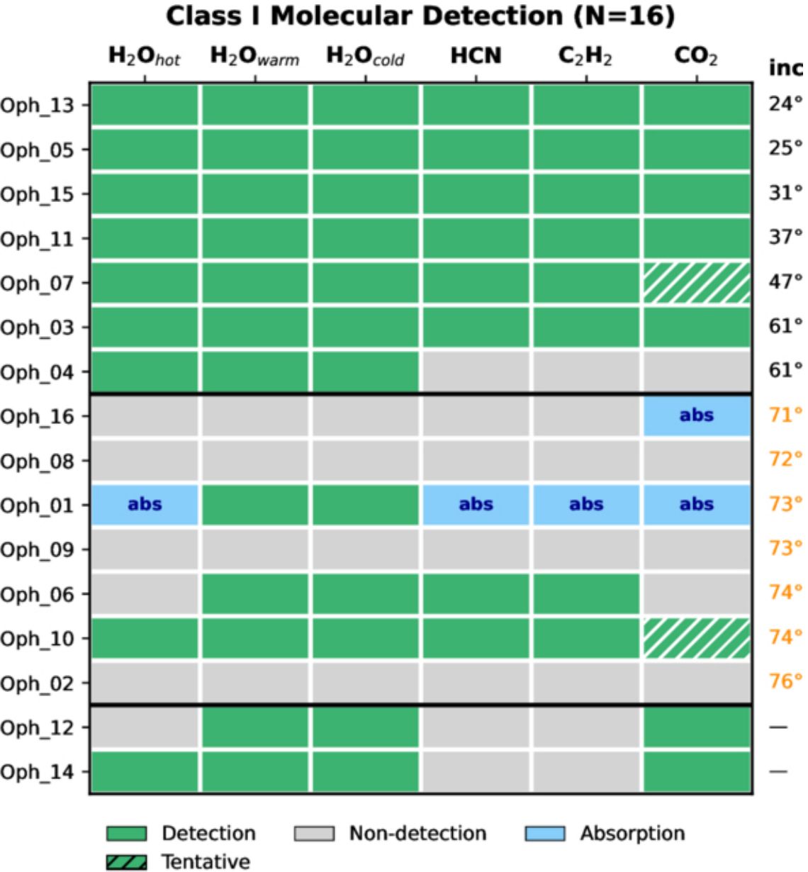
Figure 3. from Ke Zhang et al 2026 Astron. J. 172 doi:10.3847/1538-3881/ae90a1 https://dx.doi.org/10.3847/1538-3881/ae90a1 © 2026. The Author(s). Published by the American Astronomical Society.
