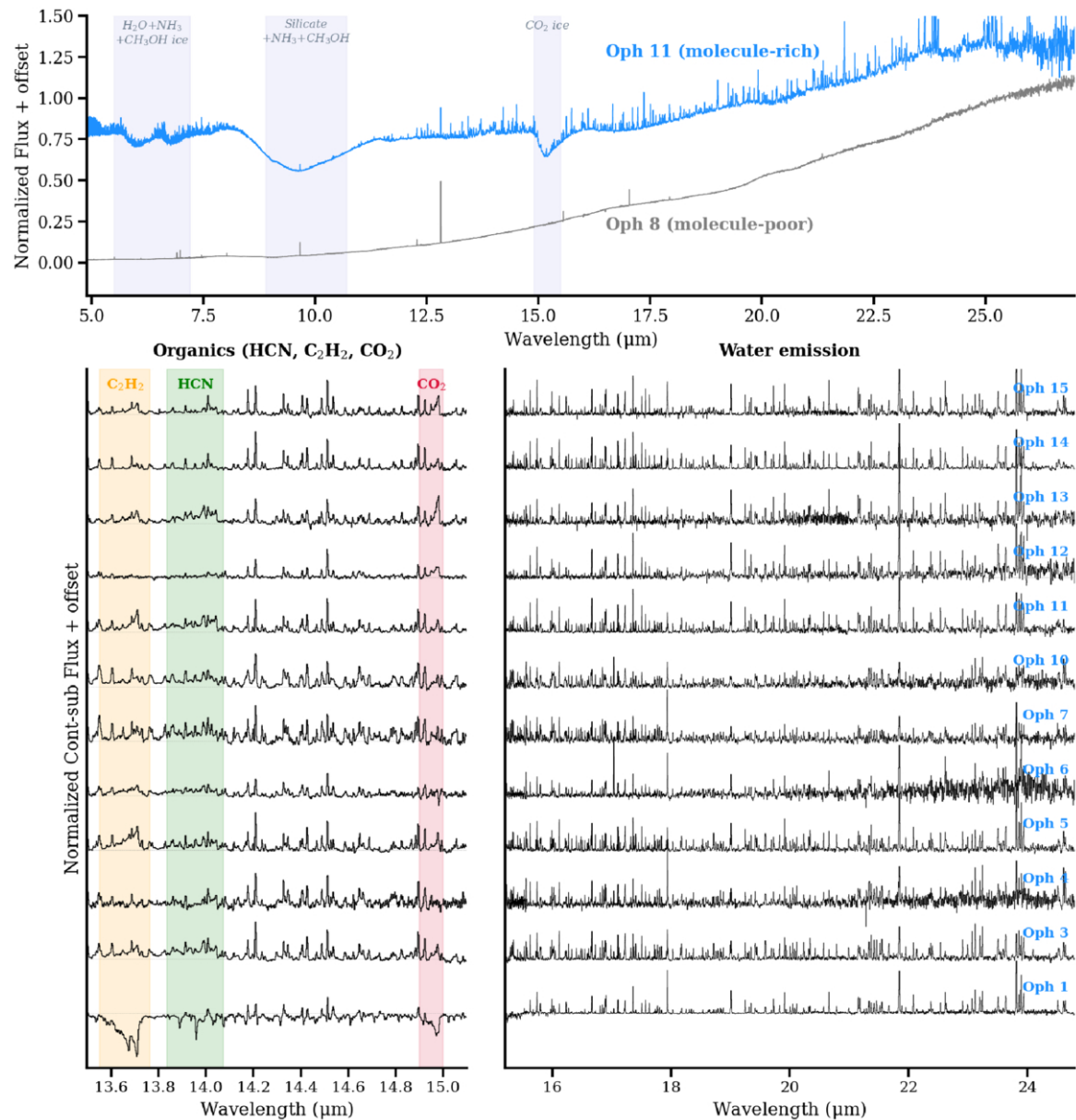
Figure 2. from Ke Zhang et al 2026 Astron. J. 172 doi:10.3847/1538-3881/ae90a1 https://dx.doi.org/10.3847/1538-3881/ae90a1 © 2026. The Author(s). Published by the American Astronomical Society.
