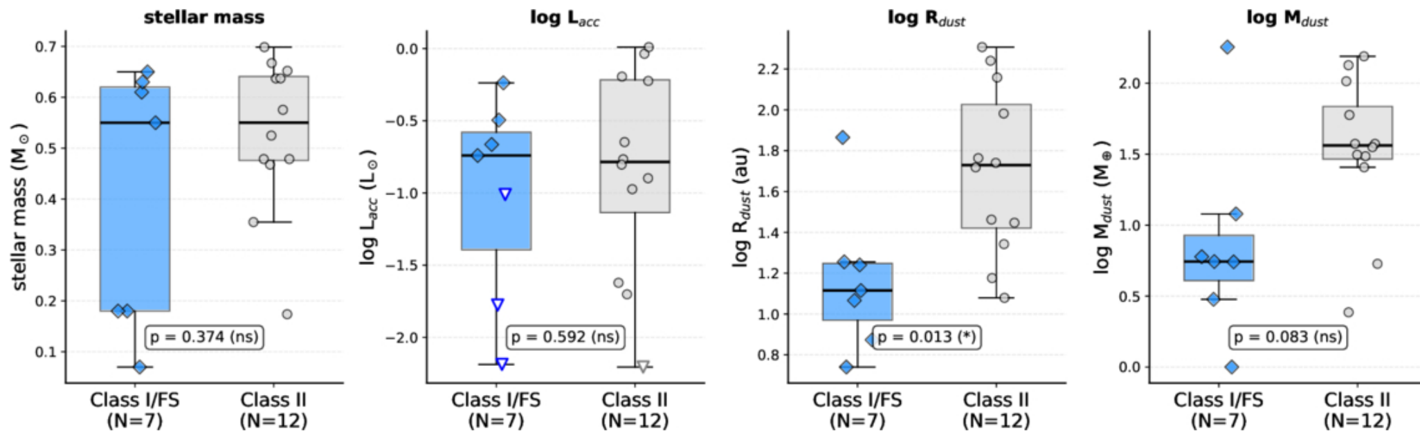
Figure 1. from Ke Zhang et al 2026 Astron. J. 172 doi:10.3847/1538-3881/ae90a1 https://dx.doi.org/10.3847/1538-3881/ae90a1 © 2026. The Author(s). Published by the American Astronomical Society.
