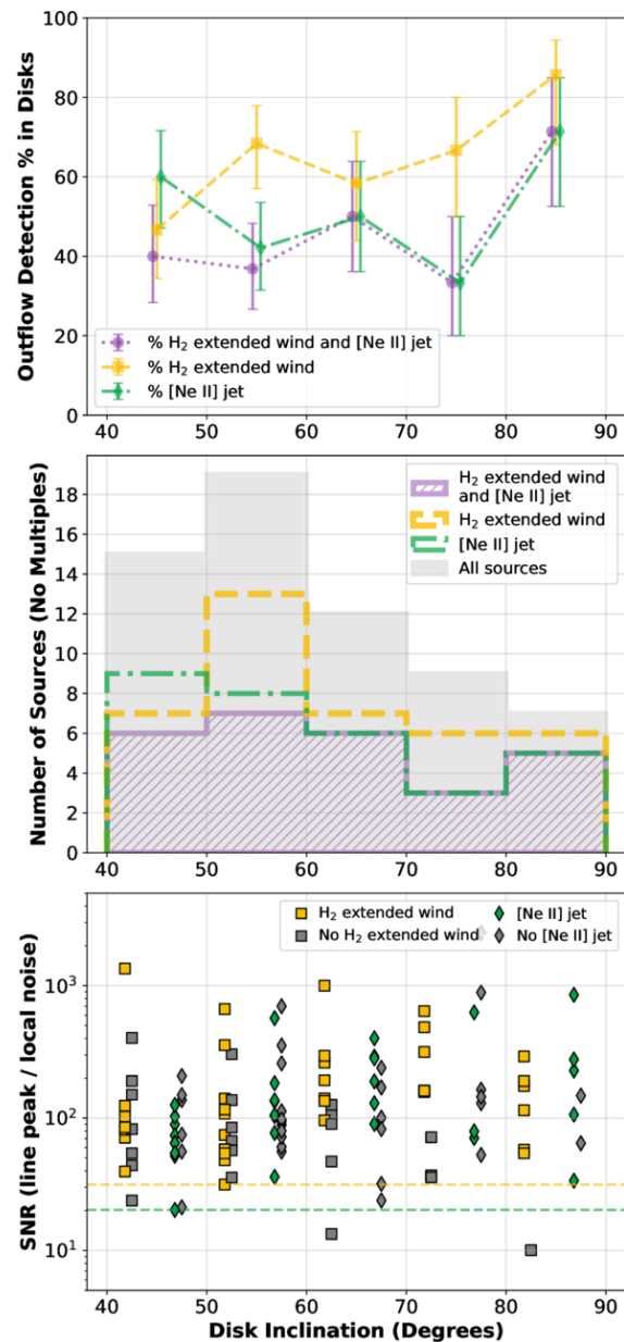
Figure 9. from Naman S. Bajaj et al 2026 Astron. J. 172 doi:10.3847/1538-3881/ae9089 https://dx.doi.org/10.3847/1538-3881/ae9089 © 2026. The Author(s). Published by the American Astronomical Society.
