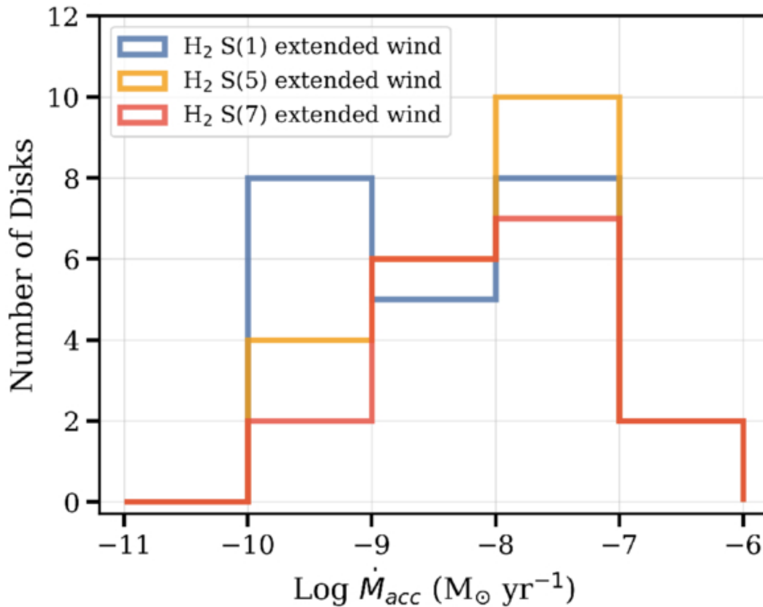
Figure 8. from Naman S. Bajaj et al 2026 Astron. J. 172 doi:10.3847/1538-3881/ae9089 https://dx.doi.org/10.3847/1538-3881/ae9089 © 2026. The Author(s). Published by the American Astronomical Society.
