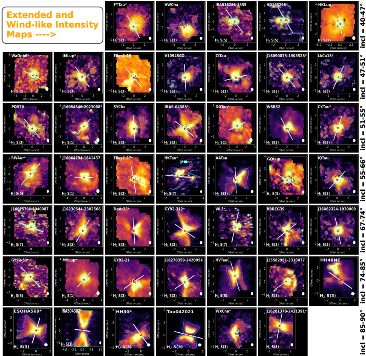
Figure 5. from Naman S. Bajaj et al 2026 Astron. J. 172 doi:10.3847/1538-3881/ae9089 https://dx.doi.org/10.3847/1538-3881/ae9089 © 2026. The Author(s). Published by the American Astronomical Society.
