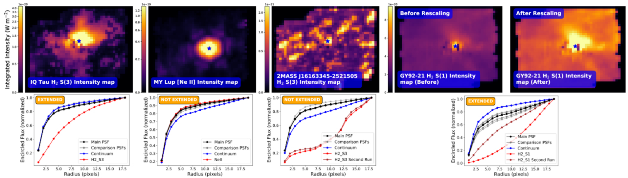
Figure 2. from Naman S. Bajaj et al 2026 Astron. J. 172 doi:10.3847/1538-3881/ae9089 https://dx.doi.org/10.3847/1538-3881/ae9089 © 2026. The Author(s). Published by the American Astronomical Society.
