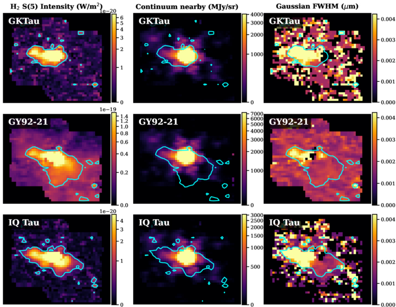
Figure 15. from Naman S. Bajaj et al 2026 Astron. J. 172 doi:10.3847/1538-3881/ae9089 https://dx.doi.org/10.3847/1538-3881/ae9089 © 2026. The Author(s). Published by the American Astronomical Society.
