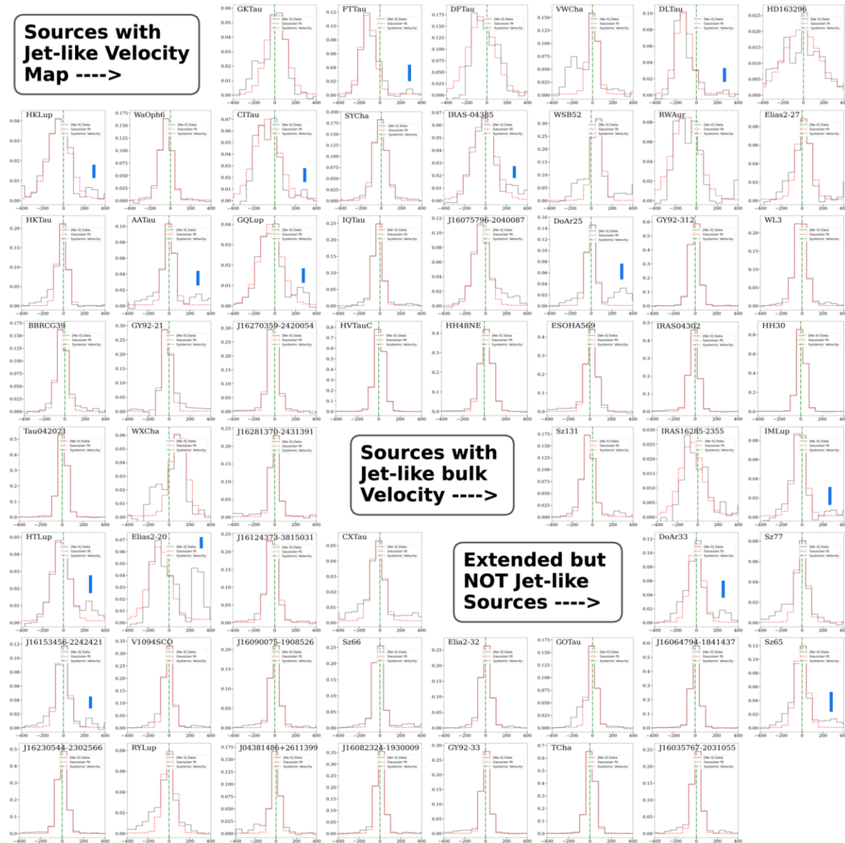
Figure 14. from Naman S. Bajaj et al 2026 Astron. J. 172 doi:10.3847/1538-3881/ae9089 https://dx.doi.org/10.3847/1538-3881/ae9089 © 2026. The Author(s). Published by the American Astronomical Society.
