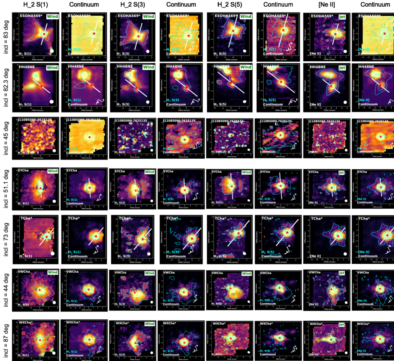
Figure 13. from Naman S. Bajaj et al 2026 Astron. J. 172 doi:10.3847/1538-3881/ae9089 https://dx.doi.org/10.3847/1538-3881/ae9089 © 2026. The Author(s). Published by the American Astronomical Society.
