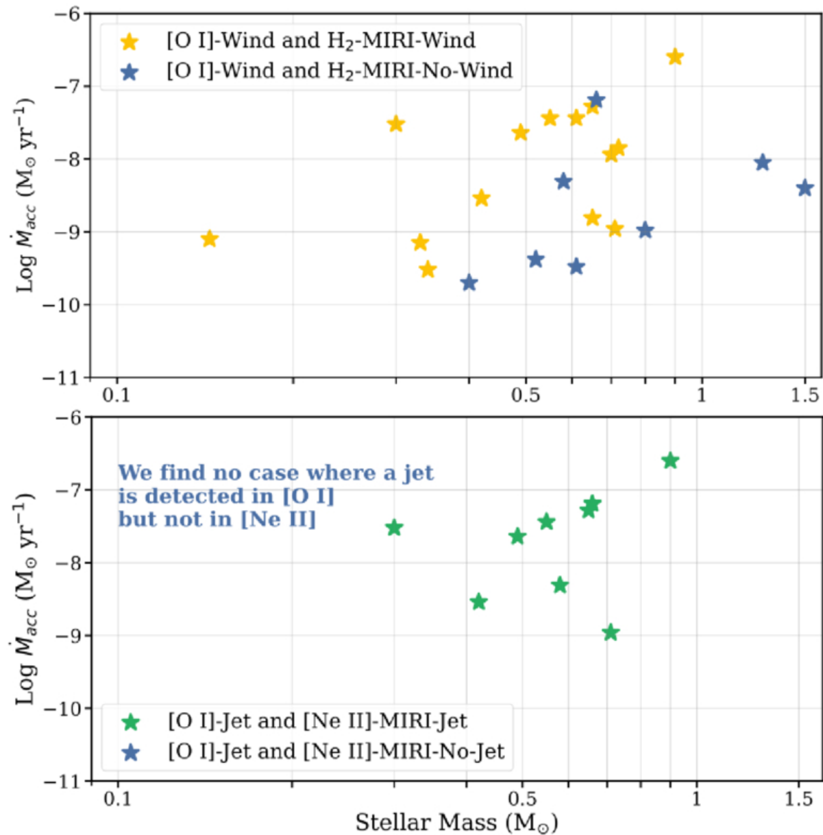
Figure 12. from Naman S. Bajaj et al 2026 Astron. J. 172 doi:10.3847/1538-3881/ae9089 https://dx.doi.org/10.3847/1538-3881/ae9089 © 2026. The Author(s). Published by the American Astronomical Society.
