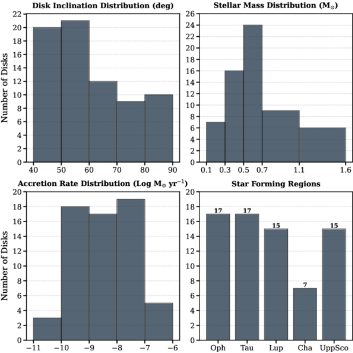
Figure 1. from Naman S. Bajaj et al 2026 Astron. J. 172 doi:10.3847/1538-3881/ae9089 https://dx.doi.org/10.3847/1538-3881/ae9089 © 2026. The Author(s). Published by the American Astronomical Society.
