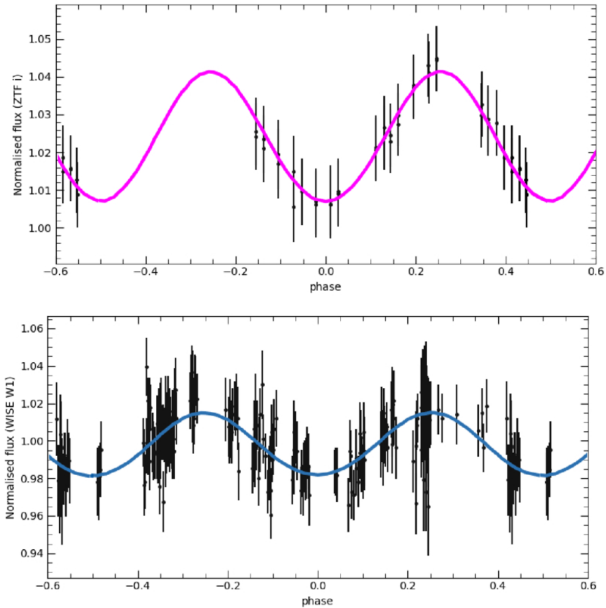
Figure 8. from Mikhail Yu. Kovalev et al 2026 Astron. J. 172 doi:10.3847/1538-3881/ae9086 https://dx.doi.org/10.3847/1538-3881/ae9086 © 2026. The Author(s). Published by the American Astronomical Society.
