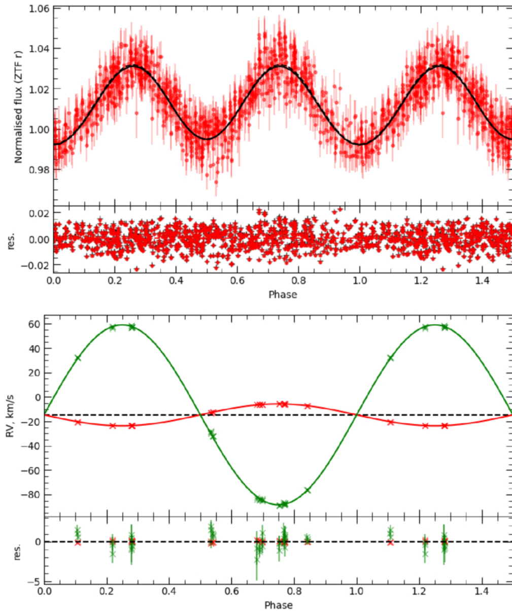
Figure 7. from Mikhail Yu. Kovalev et al 2026 Astron. J. 172 doi:10.3847/1538-3881/ae9086 https://dx.doi.org/10.3847/1538-3881/ae9086 © 2026. The Author(s). Published by the American Astronomical Society.
