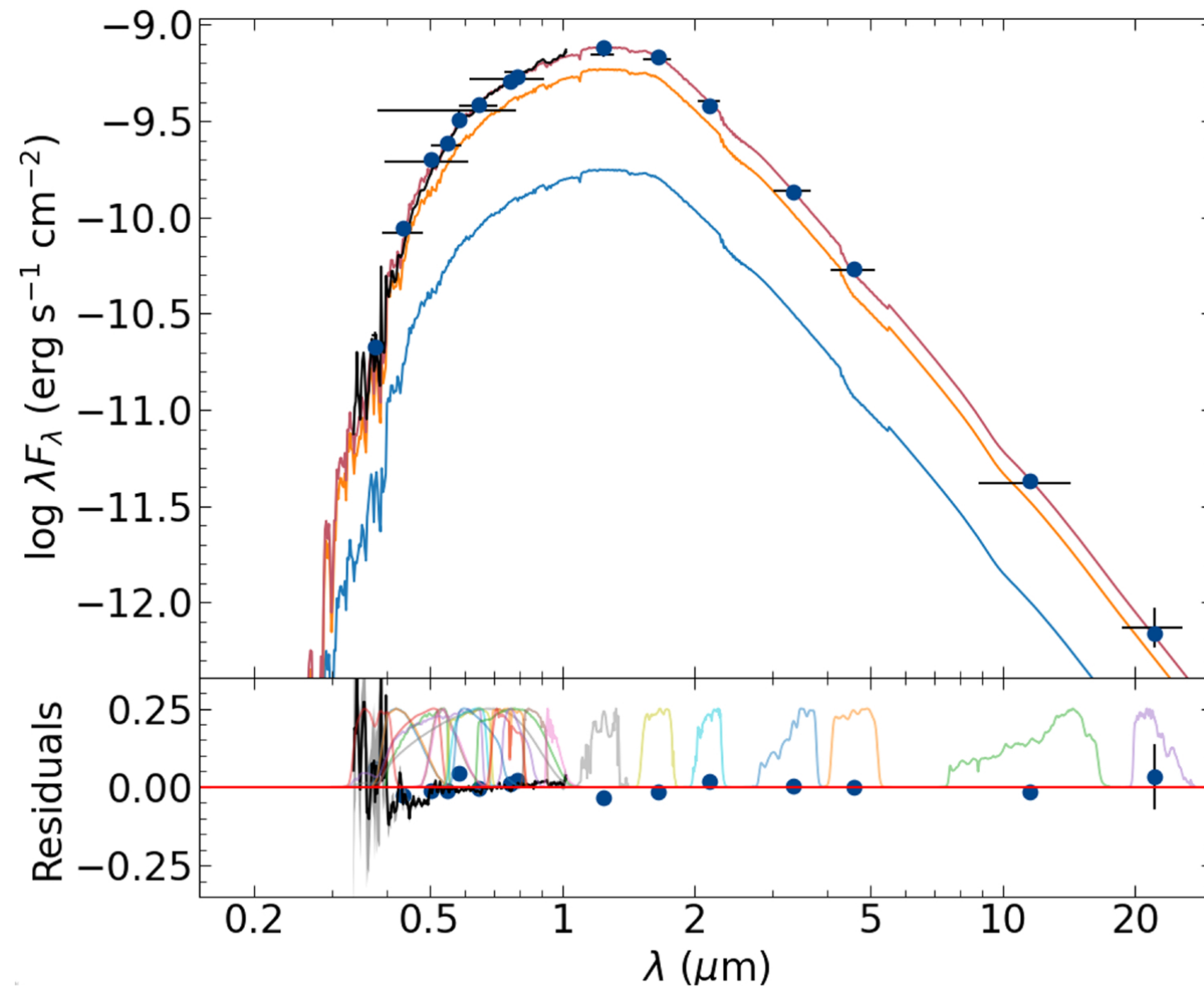
Figure 5. from Mikhail Yu. Kovalev et al 2026 Astron. J. 172 doi:10.3847/1538-3881/ae9086 https://dx.doi.org/10.3847/1538-3881/ae9086 © 2026. The Author(s). Published by the American Astronomical Society.
