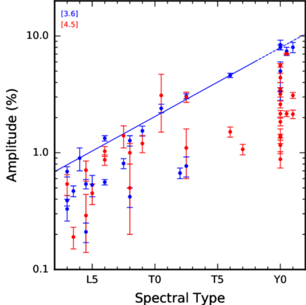
Figure 6. from Michael C. Cushing et al 2026 Astron. J. 172 doi:10.3847/1538-3881/ae8e7c https://dx.doi.org/10.3847/1538-3881/ae8e7c © 2026. The Author(s). Published by the American Astronomical Society.
