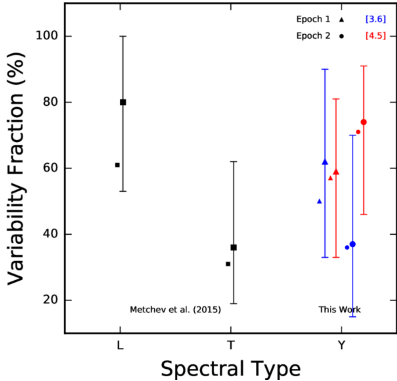
Figure 5. from Michael C. Cushing et al 2026 Astron. J. 172 doi:10.3847/1538-3881/ae8e7c https://dx.doi.org/10.3847/1538-3881/ae8e7c © 2026. The Author(s). Published by the American Astronomical Society.
