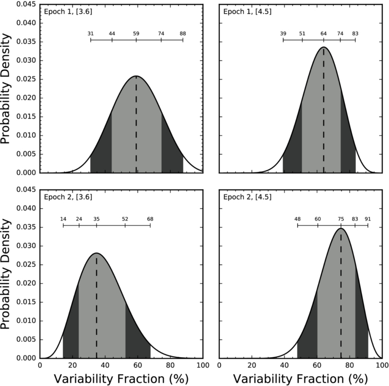
Figure 4. from Michael C. Cushing et al 2026 Astron. J. 172 doi:10.3847/1538-3881/ae8e7c https://dx.doi.org/10.3847/1538-3881/ae8e7c © 2026. The Author(s). Published by the American Astronomical Society.
