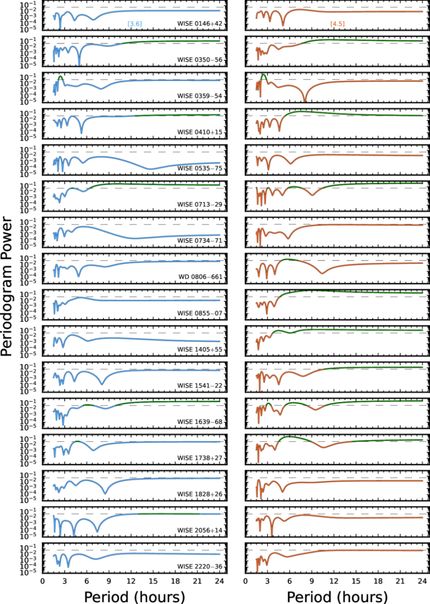
Figure 2. from Michael C. Cushing et al 2026 Astron. J. 172 doi:10.3847/1538-3881/ae8e7c https://dx.doi.org/10.3847/1538-3881/ae8e7c © 2026. The Author(s). Published by the American Astronomical Society.
