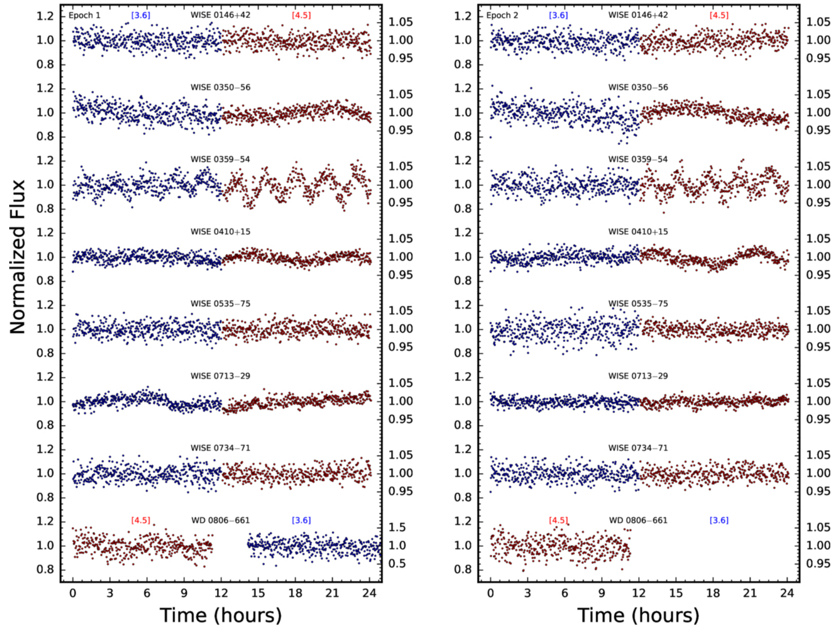
Figure 1. from Michael C. Cushing et al 2026 Astron. J. 172 doi:10.3847/1538-3881/ae8e7c https://dx.doi.org/10.3847/1538-3881/ae8e7c © 2026. The Author(s). Published by the American Astronomical Society.
