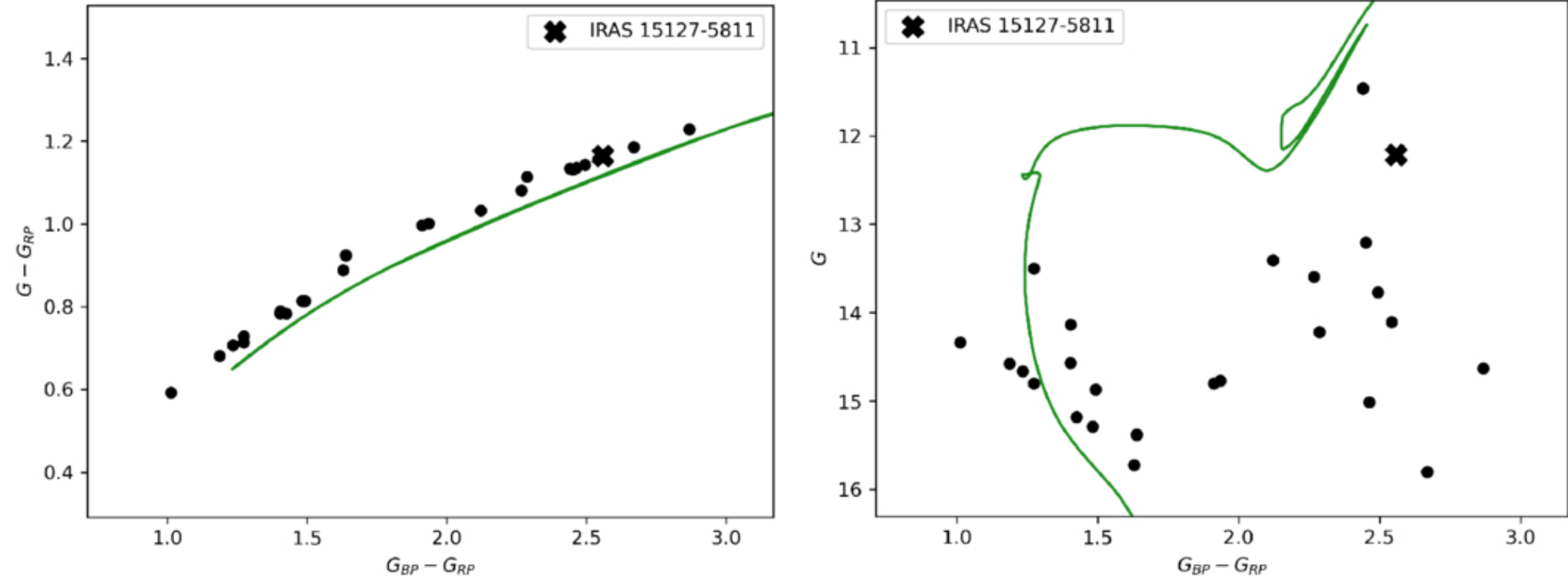
Figure A2. from Andreas Ritter et al 2026 Astron. J. 172 doi:10.3847/1538-3881/ae8db6 https://dx.doi.org/10.3847/1538-3881/ae8db6 © 2026. The Author(s). Published by the American Astronomical Society.
