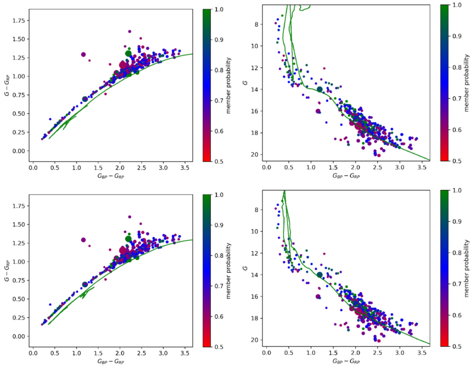
Figure 7. from Andreas Ritter et al 2026 Astron. J. 172 doi:10.3847/1538-3881/ae8db6 https://dx.doi.org/10.3847/1538-3881/ae8db6 © 2026. The Author(s). Published by the American Astronomical Society.
