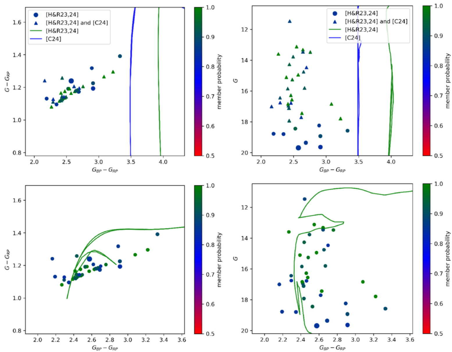
Figure 5. from Andreas Ritter et al 2026 Astron. J. 172 doi:10.3847/1538-3881/ae8db6 https://dx.doi.org/10.3847/1538-3881/ae8db6 © 2026. The Author(s). Published by the American Astronomical Society.
