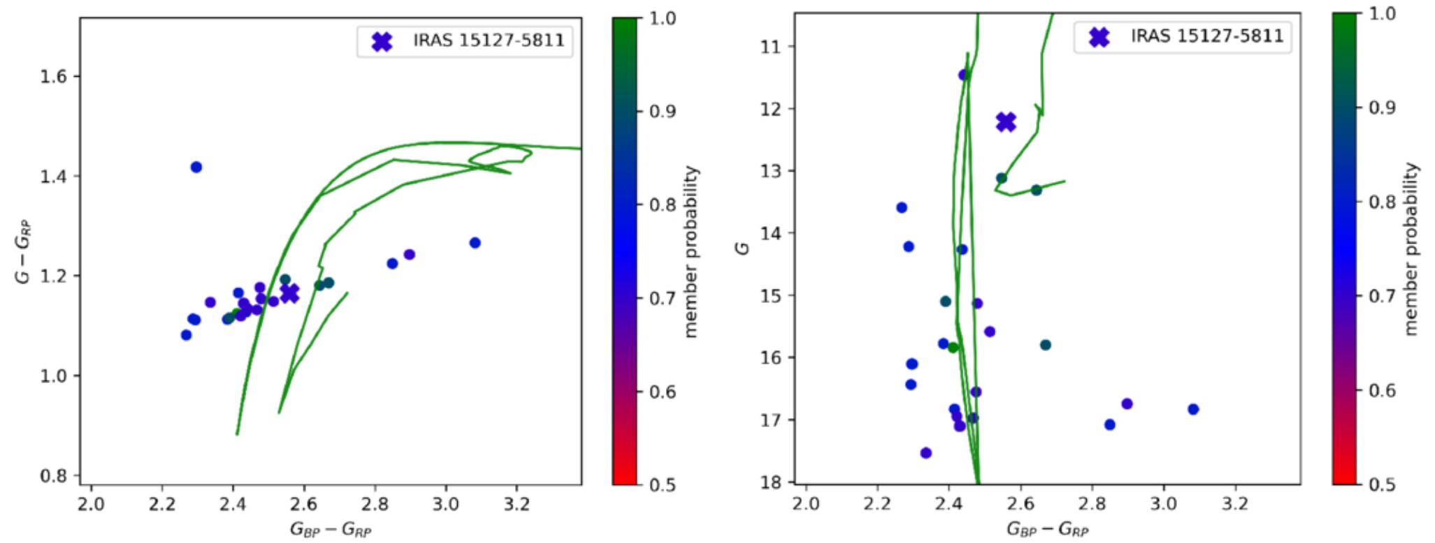
Figure A6. from Andreas Ritter et al 2026 Astron. J. 172 doi:10.3847/1538-3881/ae8db6 https://dx.doi.org/10.3847/1538-3881/ae8db6 © 2026. The Author(s). Published by the American Astronomical Society.
