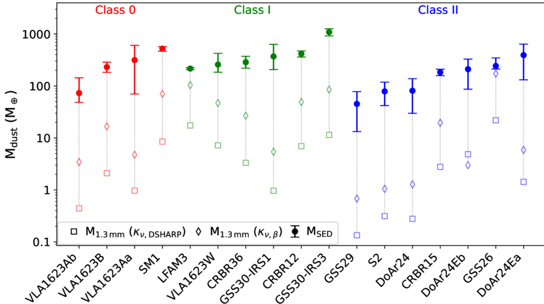
Figure 7. from Isaac C. Radley et al 2026 Astron. J. 172 doi:10.3847/1538-3881/ae8d0b https://dx.doi.org/10.3847/1538-3881/ae8d0b © 2026. The Author(s). Published by the American Astronomical Society.
