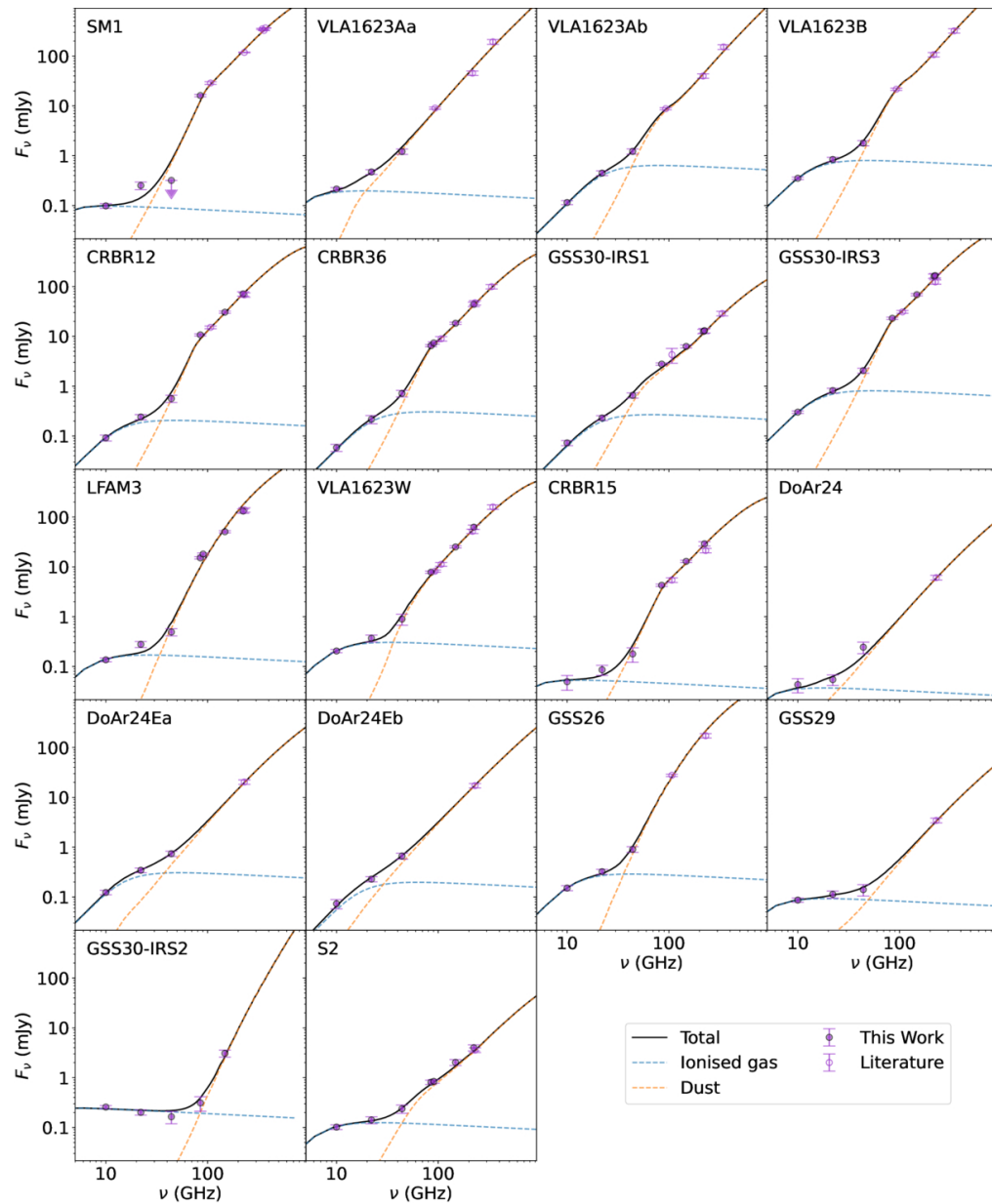
Figure 6. from Isaac C. Radley et al 2026 Astron. J. 172 doi:10.3847/1538-3881/ae8d0b https://dx.doi.org/10.3847/1538-3881/ae8d0b © 2026. The Author(s). Published by the American Astronomical Society.
