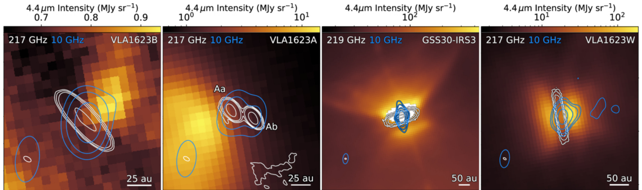
Figure 3. from Isaac C. Radley et al 2026 Astron. J. 172 doi:10.3847/1538-3881/ae8d0b https://dx.doi.org/10.3847/1538-3881/ae8d0b © 2026. The Author(s). Published by the American Astronomical Society.
