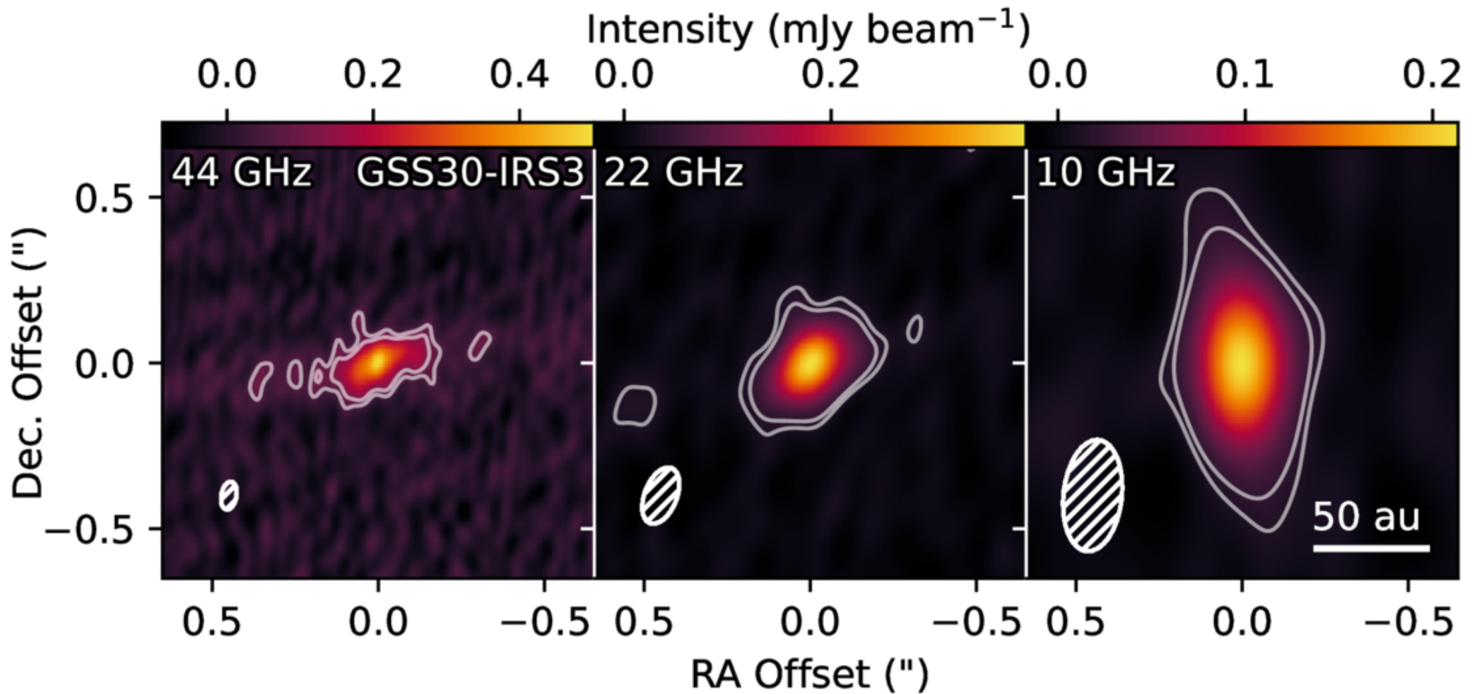
Figure 2. from Isaac C. Radley et al 2026 Astron. J. 172 doi:10.3847/1538-3881/ae8d0b https://dx.doi.org/10.3847/1538-3881/ae8d0b © 2026. The Author(s). Published by the American Astronomical Society.
