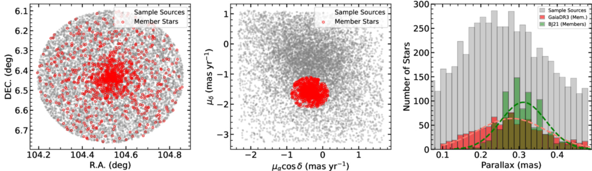
Figure 1. from D. C. Çınar et al 2026 Astron. J. 172 doi:10.3847/1538-3881/ae8d05 https://dx.doi.org/10.3847/1538-3881/ae8d05 © 2026. The Author(s). Published by the American Astronomical Society.
