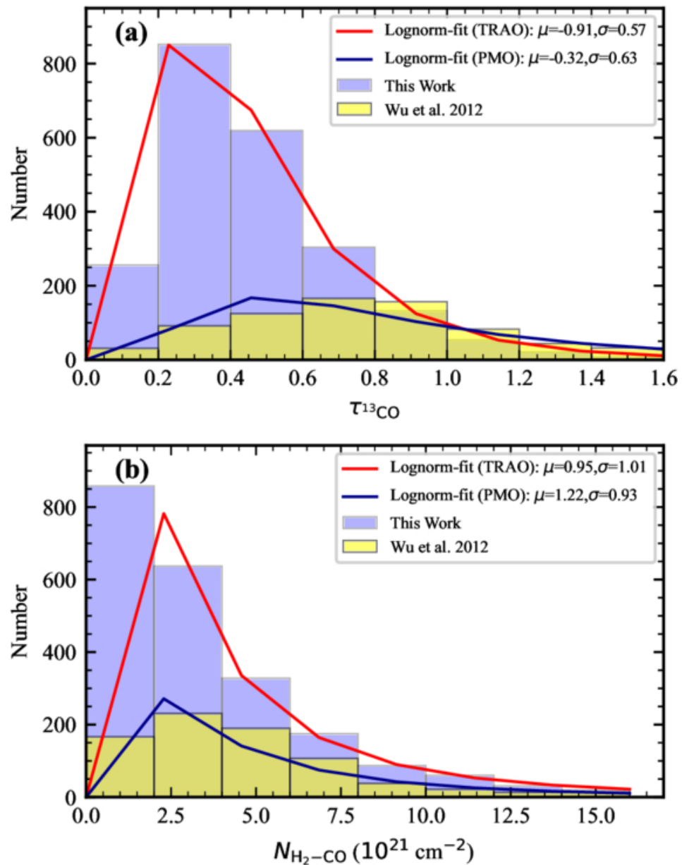
Figure 9. from Yang Yuebin et al 2026 Astron. J. 172 doi:10.3847/1538-3881/ae8cff https://dx.doi.org/10.3847/1538-3881/ae8cff © 2026. The Author(s). Published by the American Astronomical Society.
