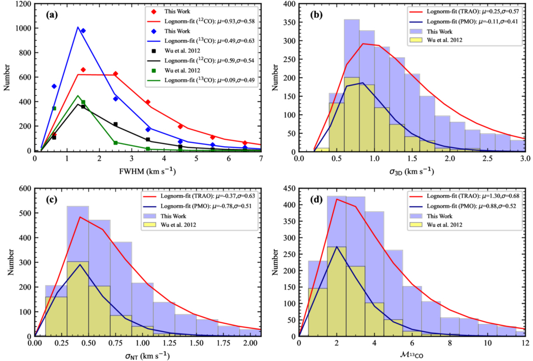
Figure 8. from Yang Yuebin et al 2026 Astron. J. 172 doi:10.3847/1538-3881/ae8cff https://dx.doi.org/10.3847/1538-3881/ae8cff © 2026. The Author(s). Published by the American Astronomical Society.
