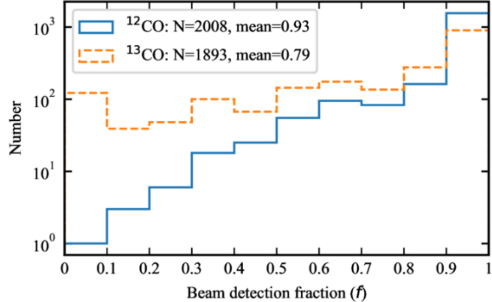
Figure 7. from Yang Yuebin et al 2026 Astron. J. 172 doi:10.3847/1538-3881/ae8cff https://dx.doi.org/10.3847/1538-3881/ae8cff © 2026. The Author(s). Published by the American Astronomical Society.
