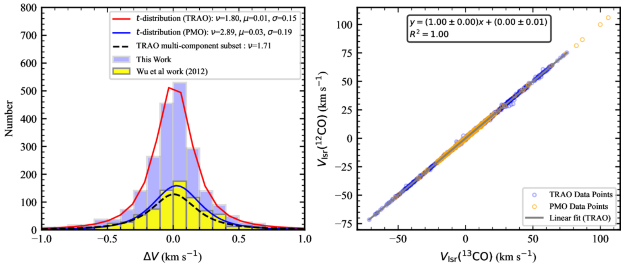
Figure 5. from Yang Yuebin et al 2026 Astron. J. 172 doi:10.3847/1538-3881/ae8cff https://dx.doi.org/10.3847/1538-3881/ae8cff © 2026. The Author(s). Published by the American Astronomical Society.
