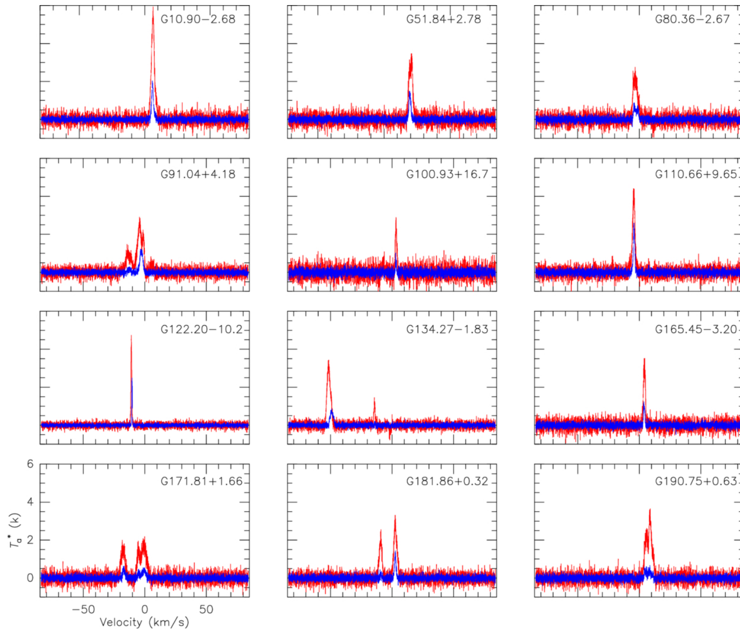
Figure 4. from Yang Yuebin et al 2026 Astron. J. 172 doi:10.3847/1538-3881/ae8cff https://dx.doi.org/10.3847/1538-3881/ae8cff © 2026. The Author(s). Published by the American Astronomical Society.
