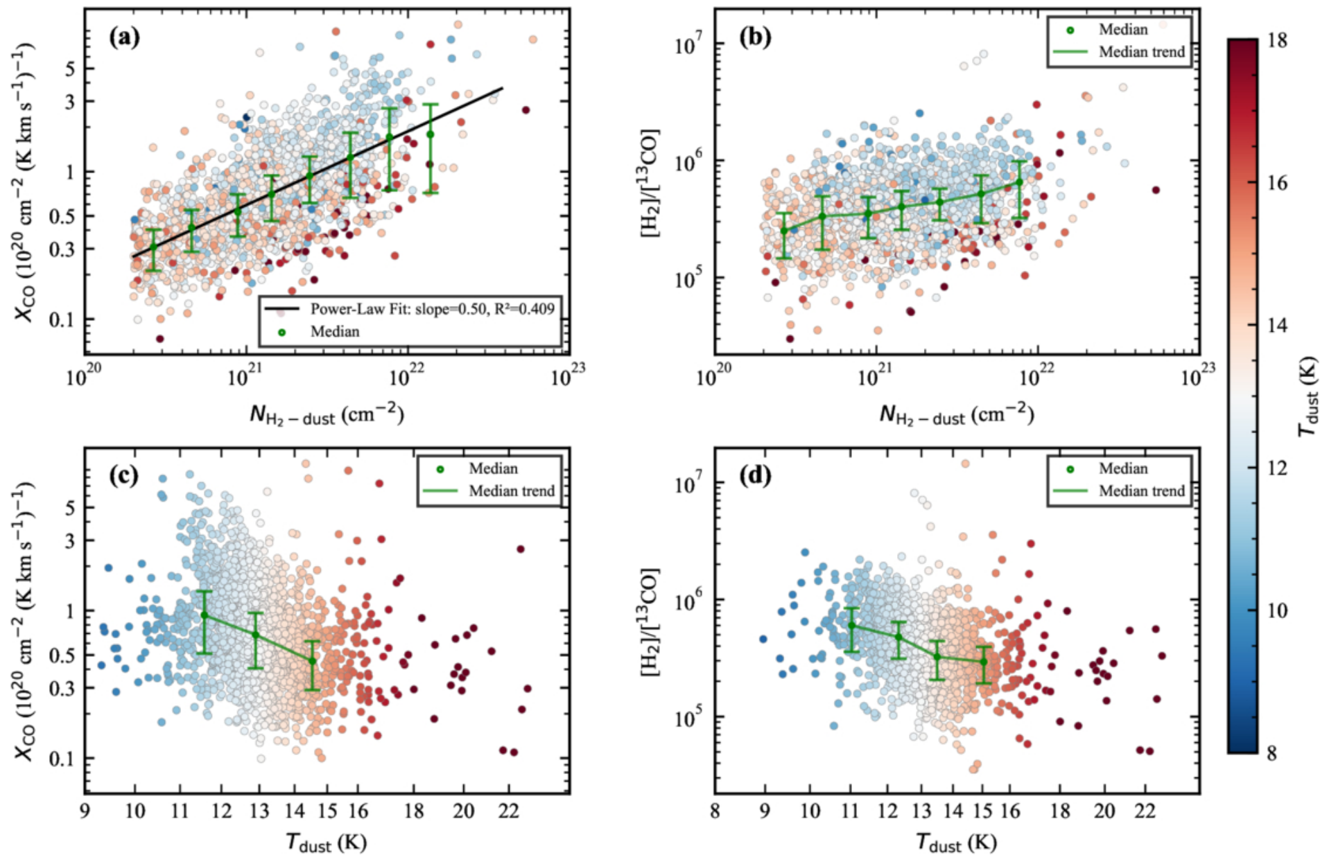
Figure 13. from Yang Yuebin et al 2026 Astron. J. 172 doi:10.3847/1538-3881/ae8cff https://dx.doi.org/10.3847/1538-3881/ae8cff © 2026. The Author(s). Published by the American Astronomical Society.
