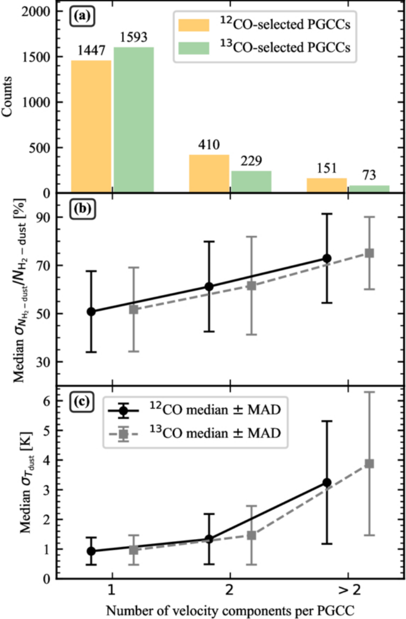
Figure 10. from Yang Yuebin et al 2026 Astron. J. 172 doi:10.3847/1538-3881/ae8cff https://dx.doi.org/10.3847/1538-3881/ae8cff © 2026. The Author(s). Published by the American Astronomical Society.
