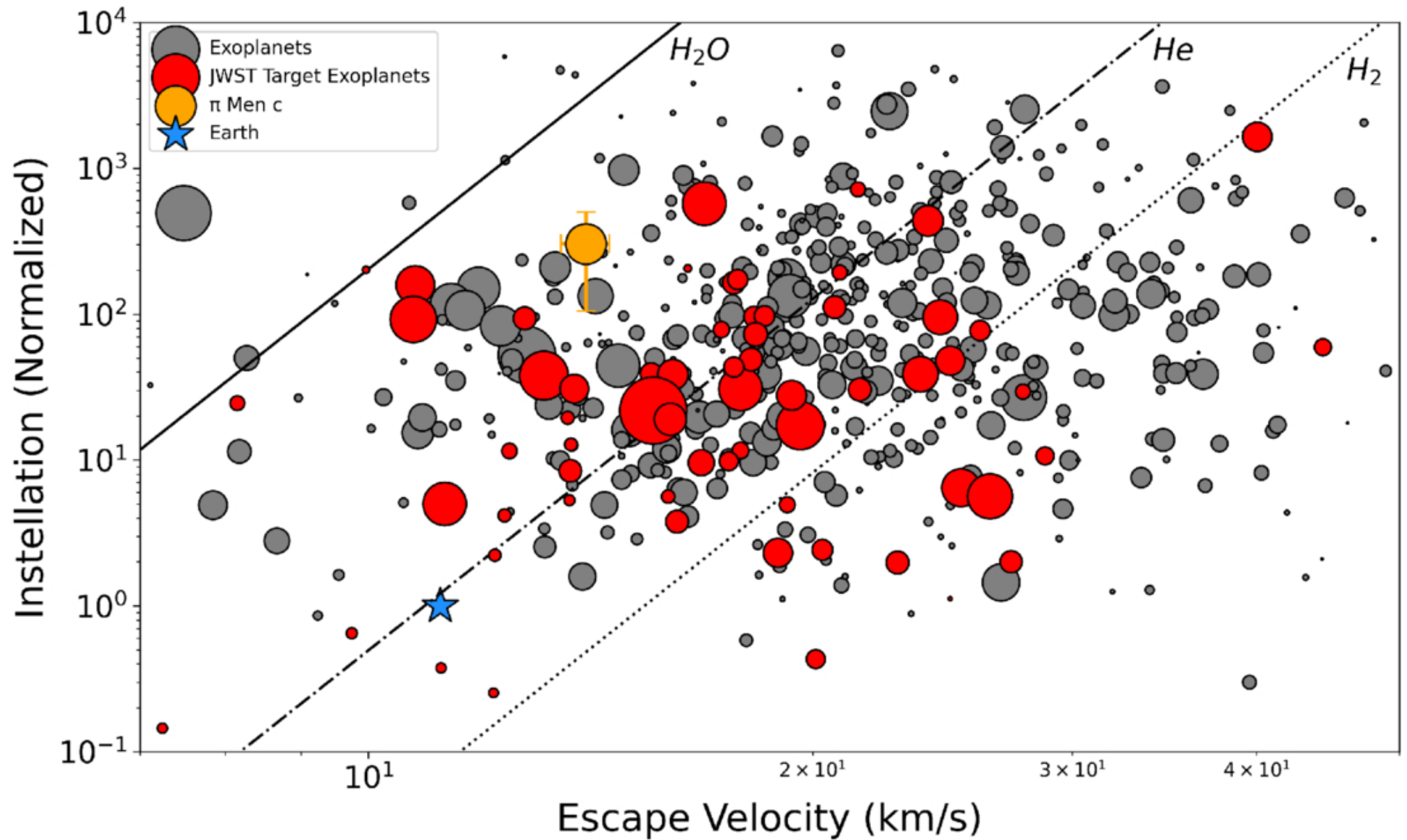
Figure 8. from Skylar S. Larsen et al 2026 Astron. J. 172 doi:10.3847/1538-3881/ae8cfb https://dx.doi.org/10.3847/1538-3881/ae8cfb © 2026. The Author(s). Published by the American Astronomical Society.
