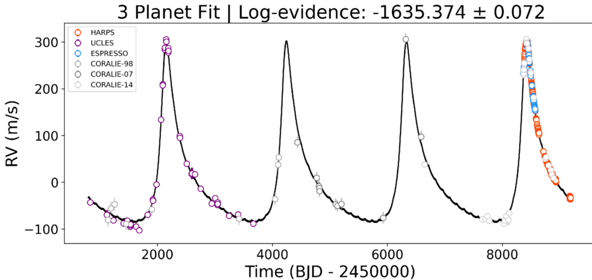
Figure 5. from Skylar S. Larsen et al 2026 Astron. J. 172 doi:10.3847/1538-3881/ae8cfb https://dx.doi.org/10.3847/1538-3881/ae8cfb © 2026. The Author(s). Published by the American Astronomical Society.
