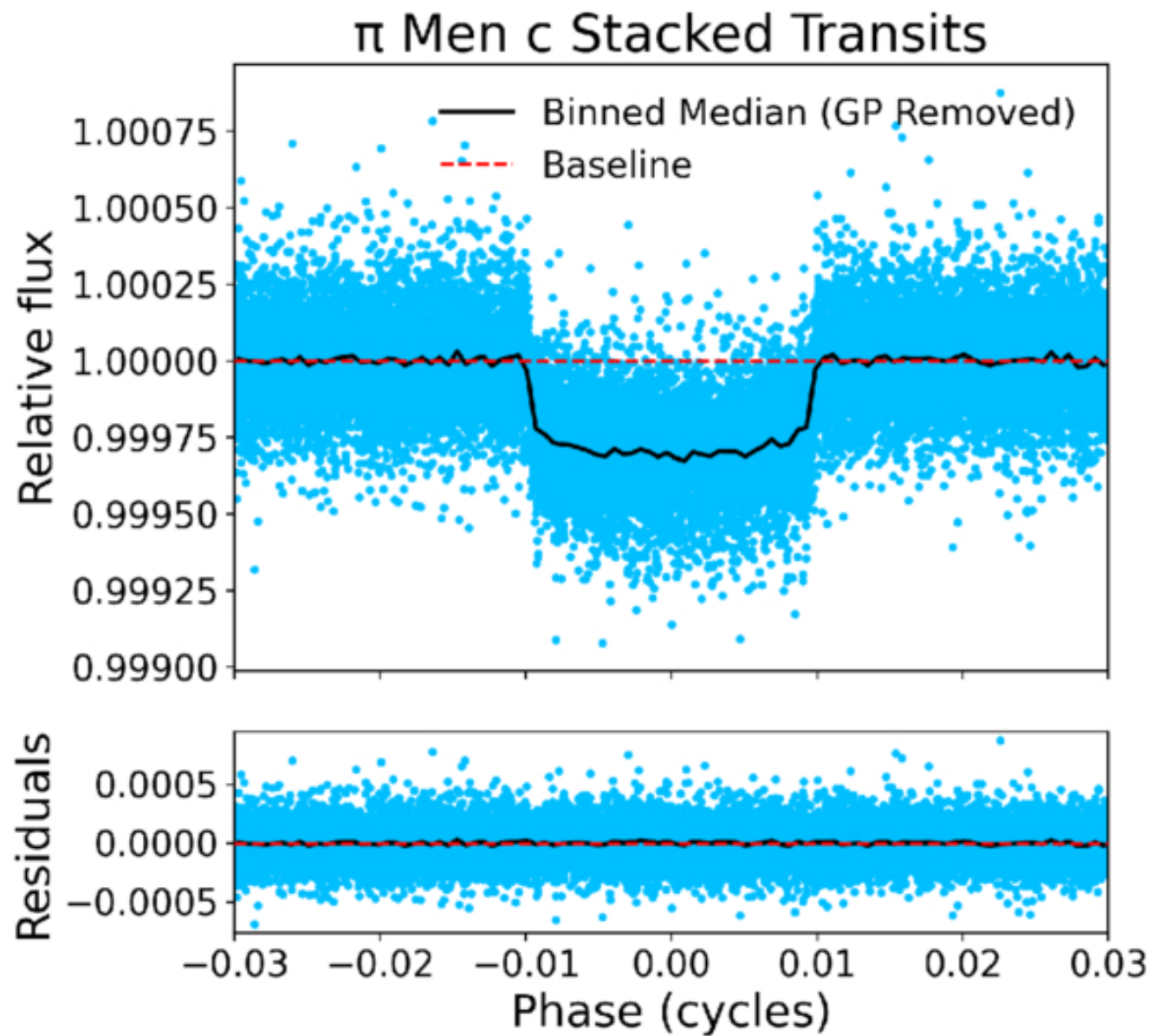
Figure 3. from Skylar S. Larsen et al 2026 Astron. J. 172 doi:10.3847/1538-3881/ae8cfb https://dx.doi.org/10.3847/1538-3881/ae8cfb © 2026. The Author(s). Published by the American Astronomical Society.
