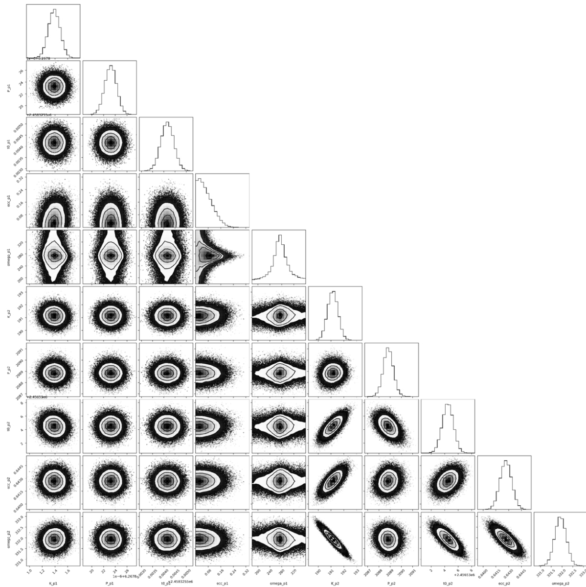
Figure 10. from Skylar S. Larsen et al 2026 Astron. J. 172 doi:10.3847/1538-3881/ae8cfb https://dx.doi.org/10.3847/1538-3881/ae8cfb © 2026. The Author(s). Published by the American Astronomical Society.
