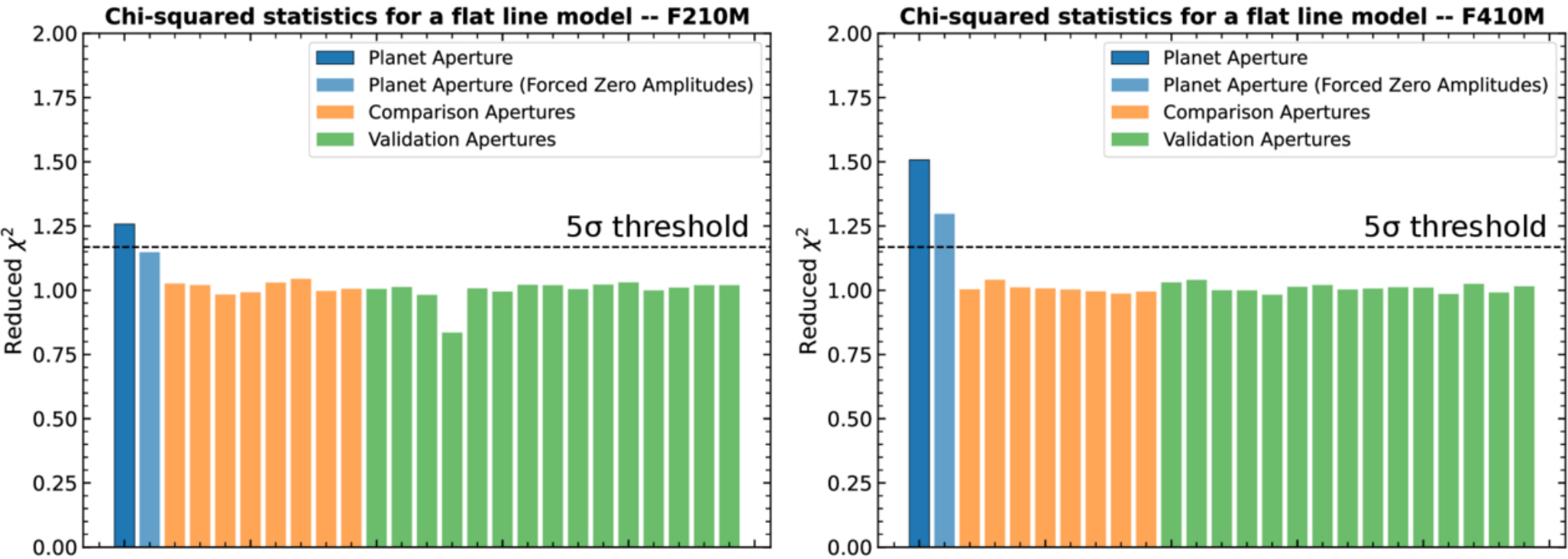
Figure 9. from Yifan Zhou et al 2026 Astron. J. 172 doi:10.3847/1538-3881/ae8bab https://dx.doi.org/10.3847/1538-3881/ae8bab © 2026. The Author(s). Published by the American Astronomical Society.
