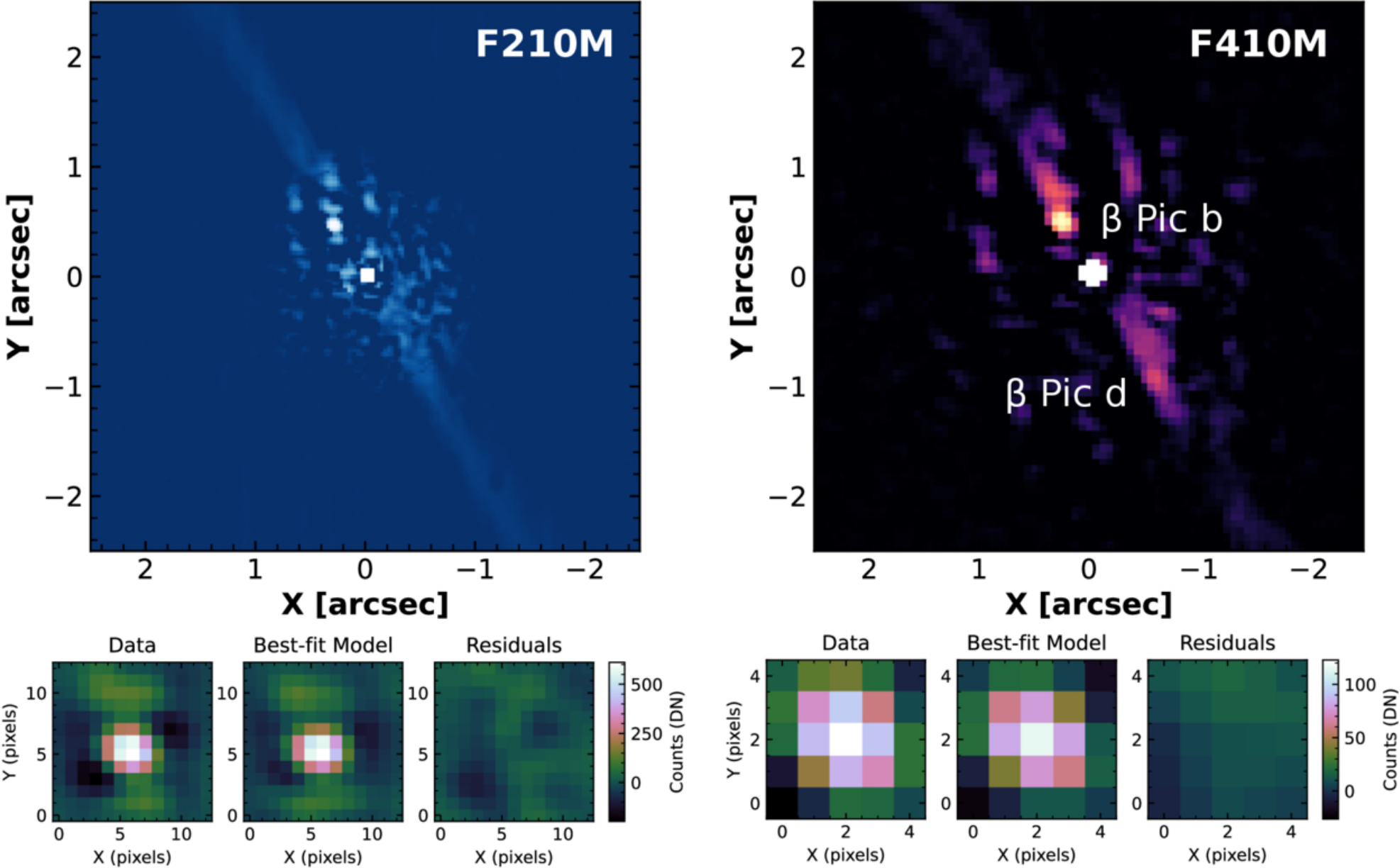
Figure 4. from Yifan Zhou et al 2026 Astron. J. 172 doi:10.3847/1538-3881/ae8bab https://dx.doi.org/10.3847/1538-3881/ae8bab © 2026. The Author(s). Published by the American Astronomical Society.
