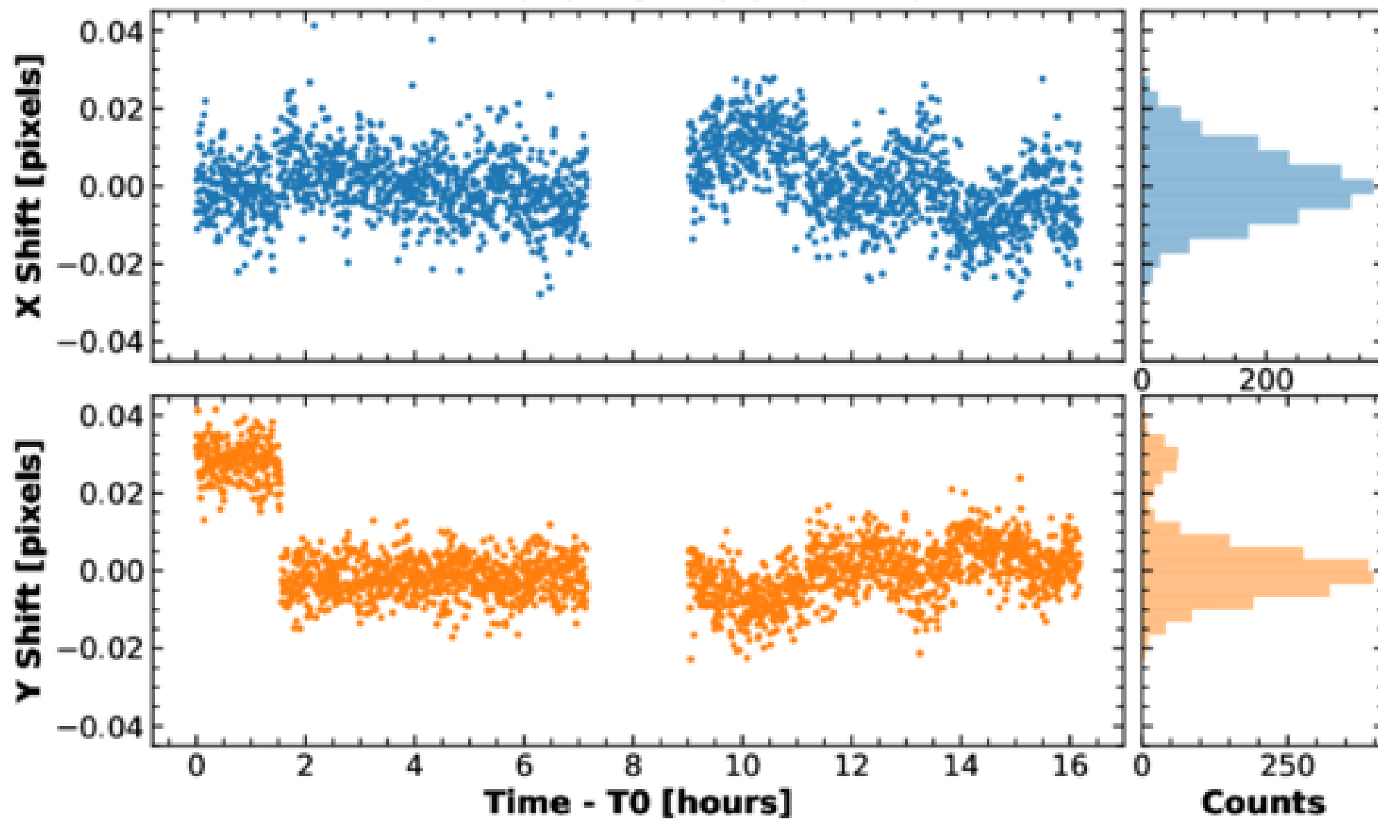
F210M X and Y Shifts Over Time
