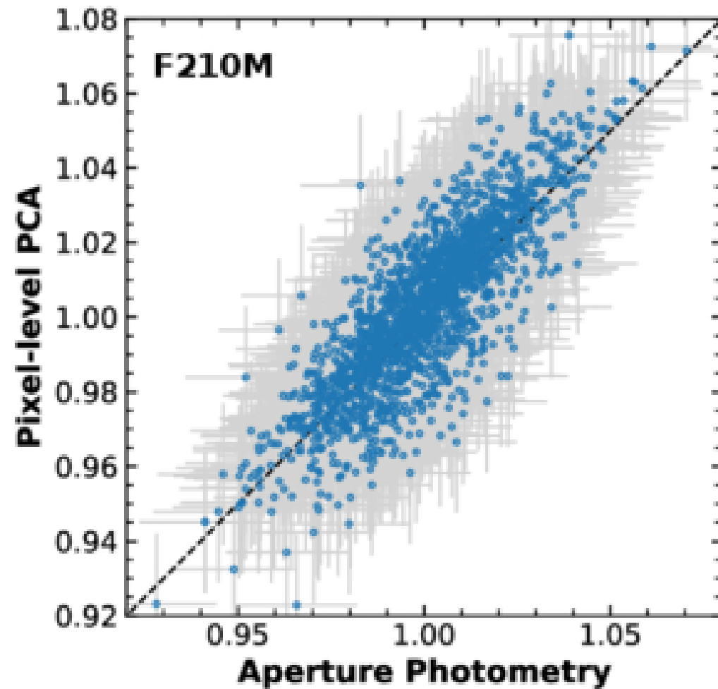
Figure 13. from Yifan Zhou et al 2026 Astron. J. 172 doi:10.3847/1538-3881/ae8bab https://dx.doi.org/10.3847/1538-3881/ae8bab © 2026. The Author(s). Published by the American Astronomical Society.
