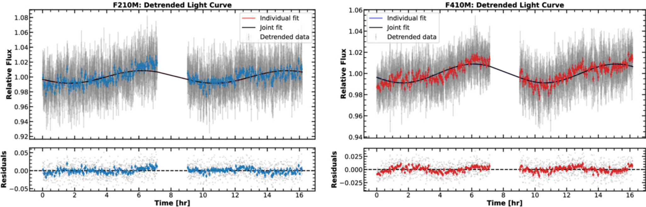
Figure 11. from Yifan Zhou et al 2026 Astron. J. 172 doi:10.3847/1538-3881/ae8bab https://dx.doi.org/10.3847/1538-3881/ae8bab © 2026. The Author(s). Published by the American Astronomical Society.
