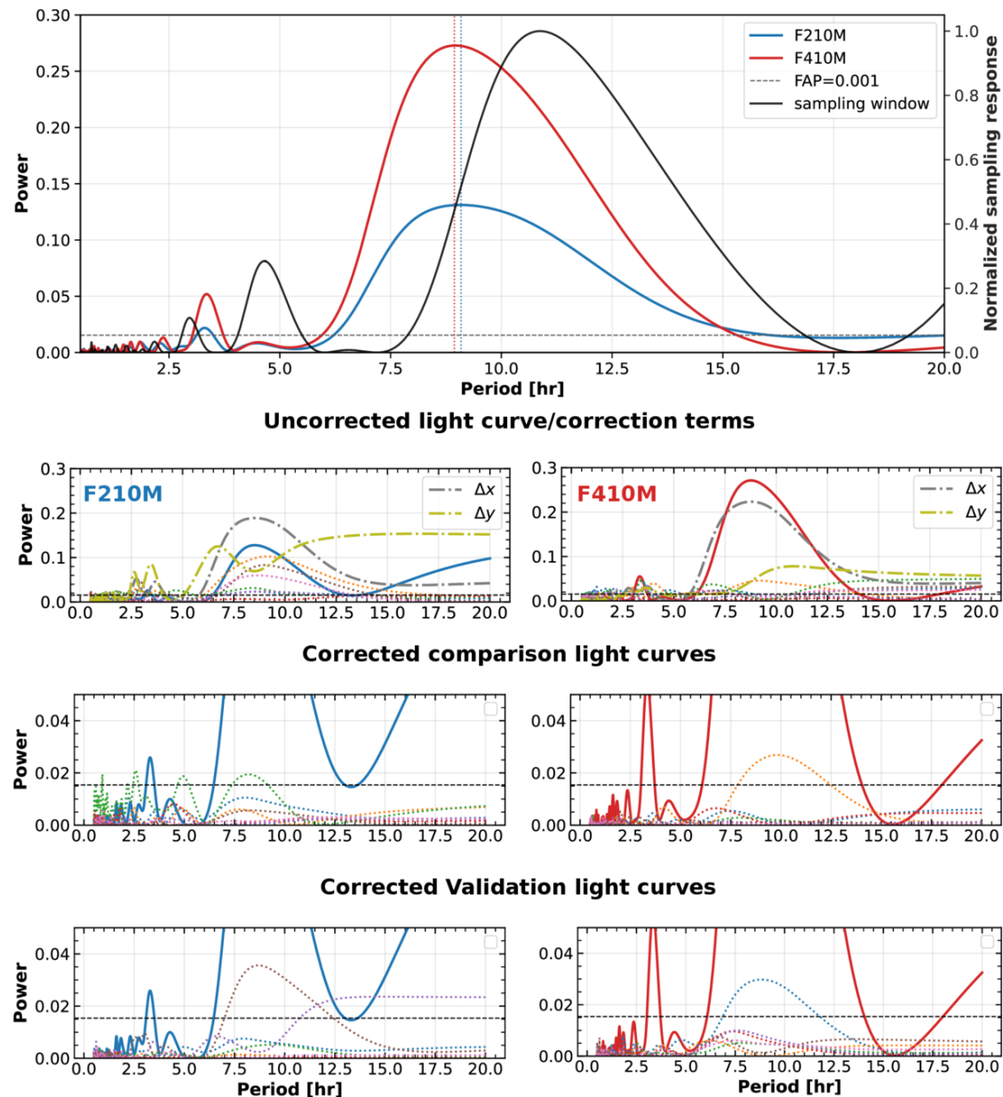
Figure 10. from Yifan Zhou et al 2026 Astron. J. 172 doi:10.3847/1538-3881/ae8bab https://dx.doi.org/10.3847/1538-3881/ae8bab © 2026. The Author(s). Published by the American Astronomical Society.
