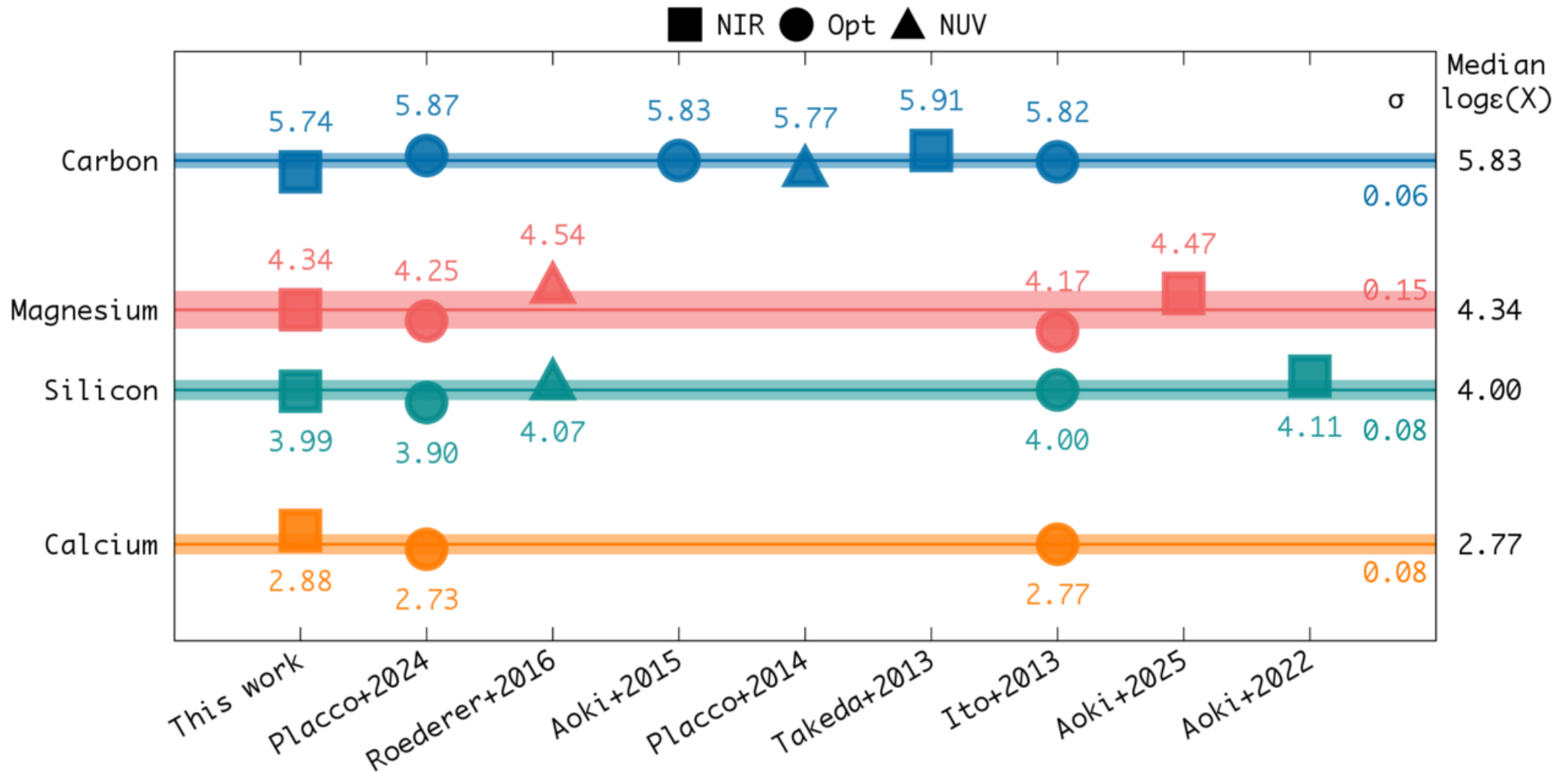
Figure 4. from Vinicius M. Placco and William D. Vacca 2026 Astron. J. 172 doi:10.3847/1538-3881/ae8b8d https://dx.doi.org/10.3847/1538-3881/ae8b8d © 2026. The Author(s). Published by the American Astronomical Society.
