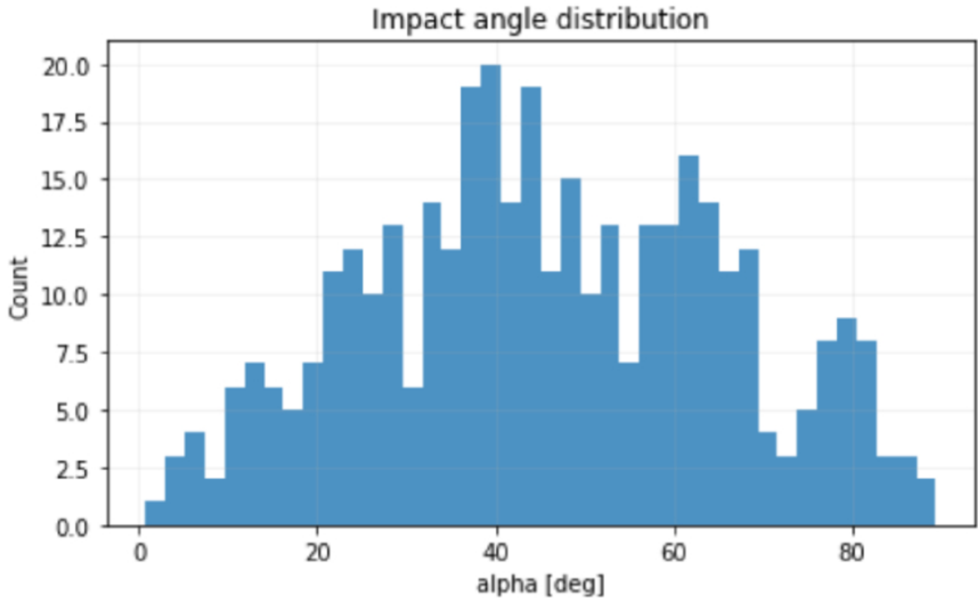
Figure 8. from Samuele Crespi et al 2026 Astron. J. 172 doi:10.3847/1538-3881/ae8ae7 https://dx.doi.org/10.3847/1538-3881/ae8ae7 © 2026. The Author(s). Published by the American Astronomical Society.
